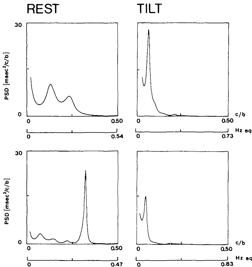
FIGURE 4. Representative example of autospectra of R-R interval variability during spontaneous breathing (top panels) and during controlled respiration, at 20/min (bottom panels). Note that, with controlled respiration at rest, the relative power of the high-frequency component becomes predominant.
