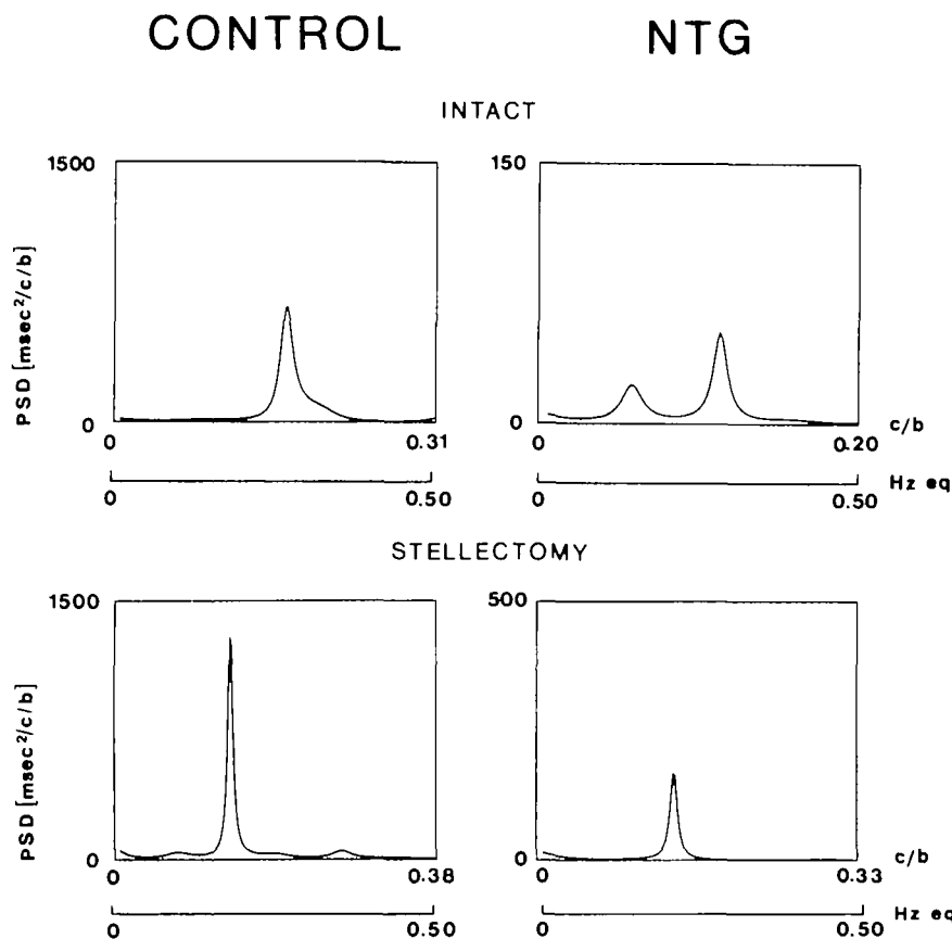
FIGURE 8. Autospectra of R-R interval variability of a conscious healthy dog in control conditions (left panels) and during an IV infusion of nitroglycerin to excite the sympathetic outflow. The top panels were obtained with cardiac nerves intact, the bottom panels after full recovery from bilateral stellectomy. Note the presence of a large low-frequency component during nitroglycerin infusion only in the neurally intact situation.
