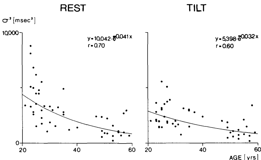
FIGURE 2. Relationship between R-R interval variability, expressed as variance ( \sigma^2 ), and age in the study population at rest and during 90° upright passive tilt. Notice that in both cases there is a significant exponential relationship ( p < 0.001 , n = 48 ).
