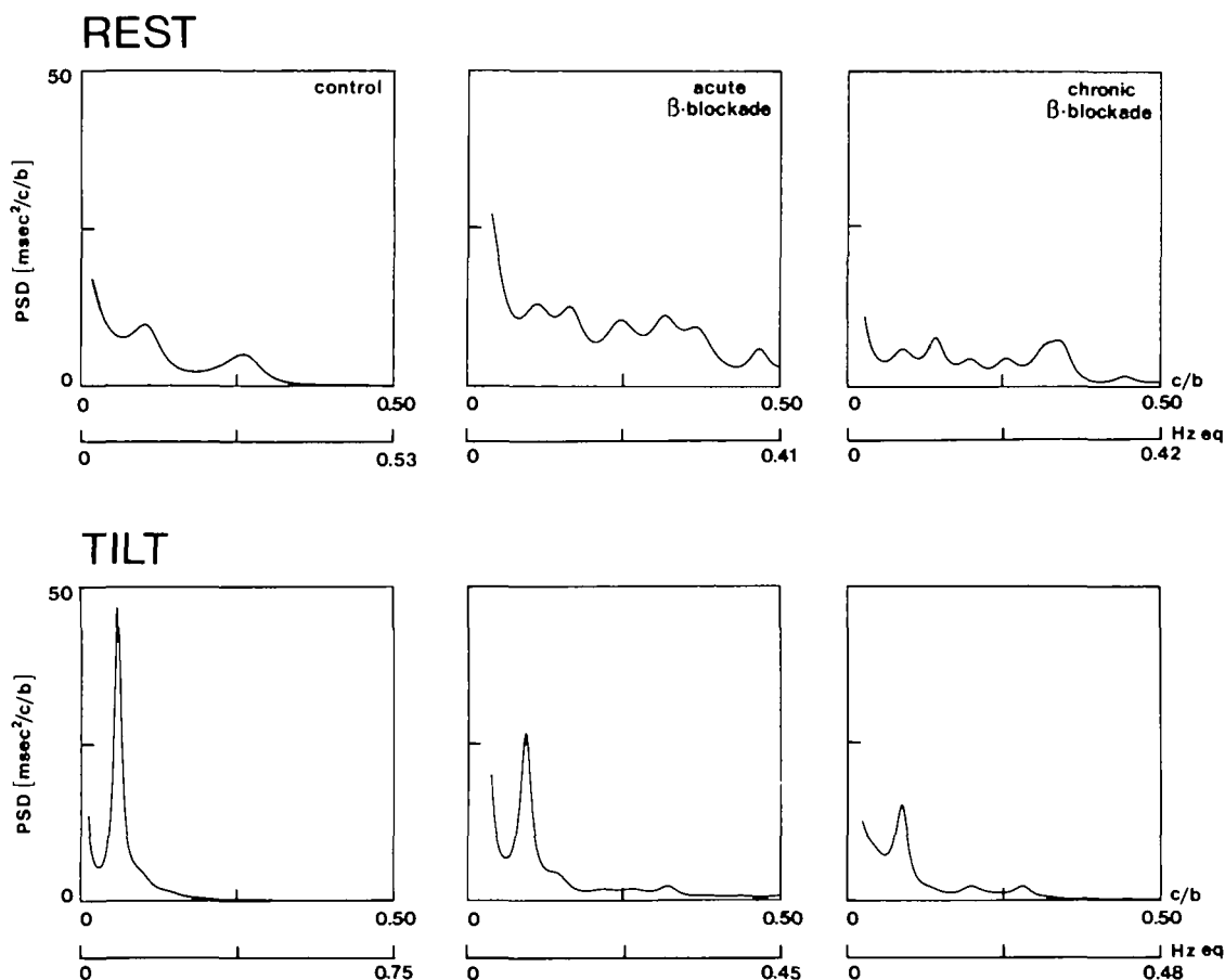
FIGURE 5. Autospectra of R-R interval variability of a young subject at rest (top panels) and during tilt (bottom panels) under control conditions (left panels) and during acute (0.2 mg/kg IV propranolol, middle panels), and chronic (0.6 mg/kg p.o. propranolol t.i.d.) \beta -adrenergic receptor blockade. Note the progressive reduction in the relative power of the low-frequency component during tilt.
