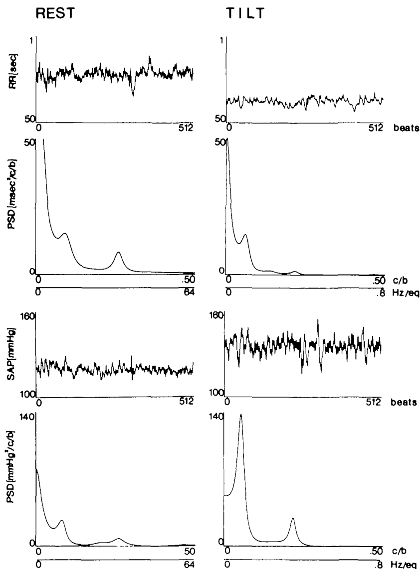
FIGURE 6. Simultaneous analysis of R-R interval and systolic arterial pressure variabilities in a young subject. Note the reduction in average R-R interval and the slight increase in average systolic arterial pressure on passing from rest to tilt. The two components of the autospectrum of systolic arterial pressure variability are similar to those of R-R interval variability at rest and during tilt.
